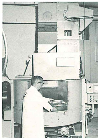
A Multi-Table is utilized for peening and blast cleaning of fragile or complex parts which cannot be tumbled.
