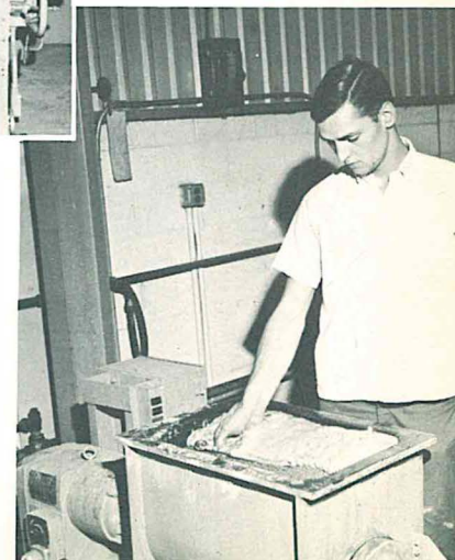
Deburring and radiusing of metal surfaces is accomplished through use of vibratory finishing equipment.
